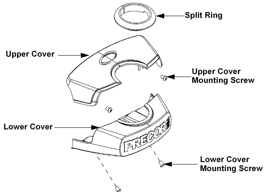
Diagram 6.1 - Mid-Point Cover
